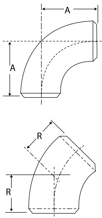
Dimensions of long radius elbows.
