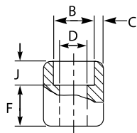
Half-Coupling
